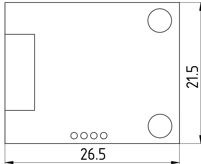
Front View (without Header Pins)
